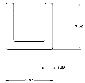
Die: 52 3/8" x 3/8" x 1/16" Channel Min. Order Qty Mtrs:475
