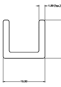
Die: 352 1/4" GLASS CHANNEL Min. Order Qty Mtrs:475
