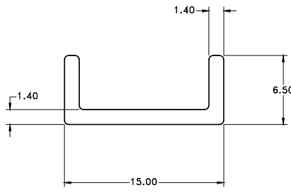
Die: 1139 15 x 6.5 x 1.4mm Channel Min. Order Qty Mtrs:525
