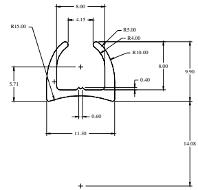
Die: 2939 Sail Track Min. Order Qty Mtrs:475
