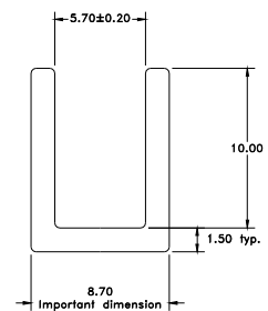
Die: 4650 Channel 8.7 x 11.5 Min. Order Qty Mtrs:425
