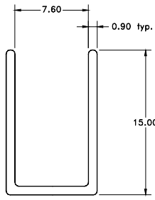
Die: 4081 7.60mm Channel Min. Order Qty Mtrs:525
