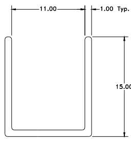
Die: 5097 Capping Channel 11mm insid Min. Order Qty Mtrs:475
