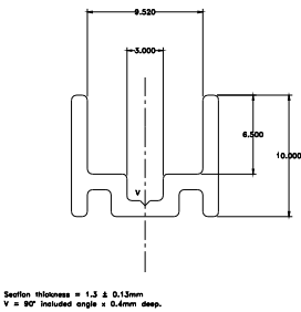
Die: 833 FLYSCREEN NO.14 Min. Order Qty Mtrs:475
